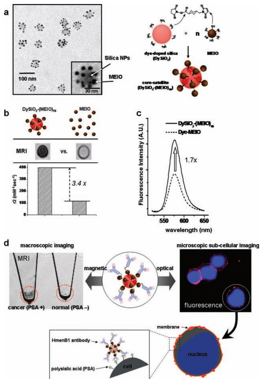
FIGURE 7. DySiO 2 -(MEIO) 10 for dual-modal MRI–optical imaging: (a) TEM and schematic diagram for the synthesis of DySiO 2 -(MEIO) 10 ; (b) synergistic MR contrast enhancement effect of DySiO 2 -(MEIO) 10 ( r_2 = 397 \text{ mM}^{-1} \text{ s}^{-1} ) with a 3.4 times higher value compared with free MEIO nanoparticles; (c) 1.7 times higher fluorescent intensity is observed for DySiO 2 -(MEIO) 10 ; (d) HmenB1 antibody conjugated DySiO 2 -(MEIO) 10 selectively detects neuroblastoma cancer cells with PSA receptors. Reproduced with permission from ref 26. Copyright 2006 Wiley-VCH.
